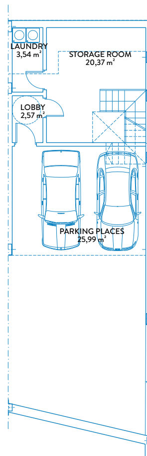
BASEMENT
