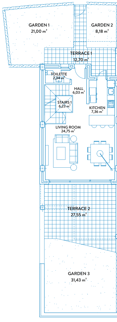
GROUND FLOOR
