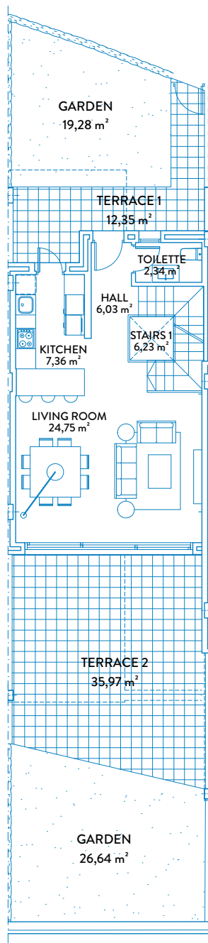
GROUND FLOOR
